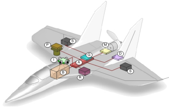
Figure 6: The Paparazzi airborne system components: (A) autopilot Control Board, (B) battery, (D) datalink Radio-Modem & Antenna, (G) GPS Receiver, (I) IR Sensors Board, (M) motor & Controller, (R) RC Receiver & Antenna, (S) servos, (P) payload = Camera & Video Transmitter
