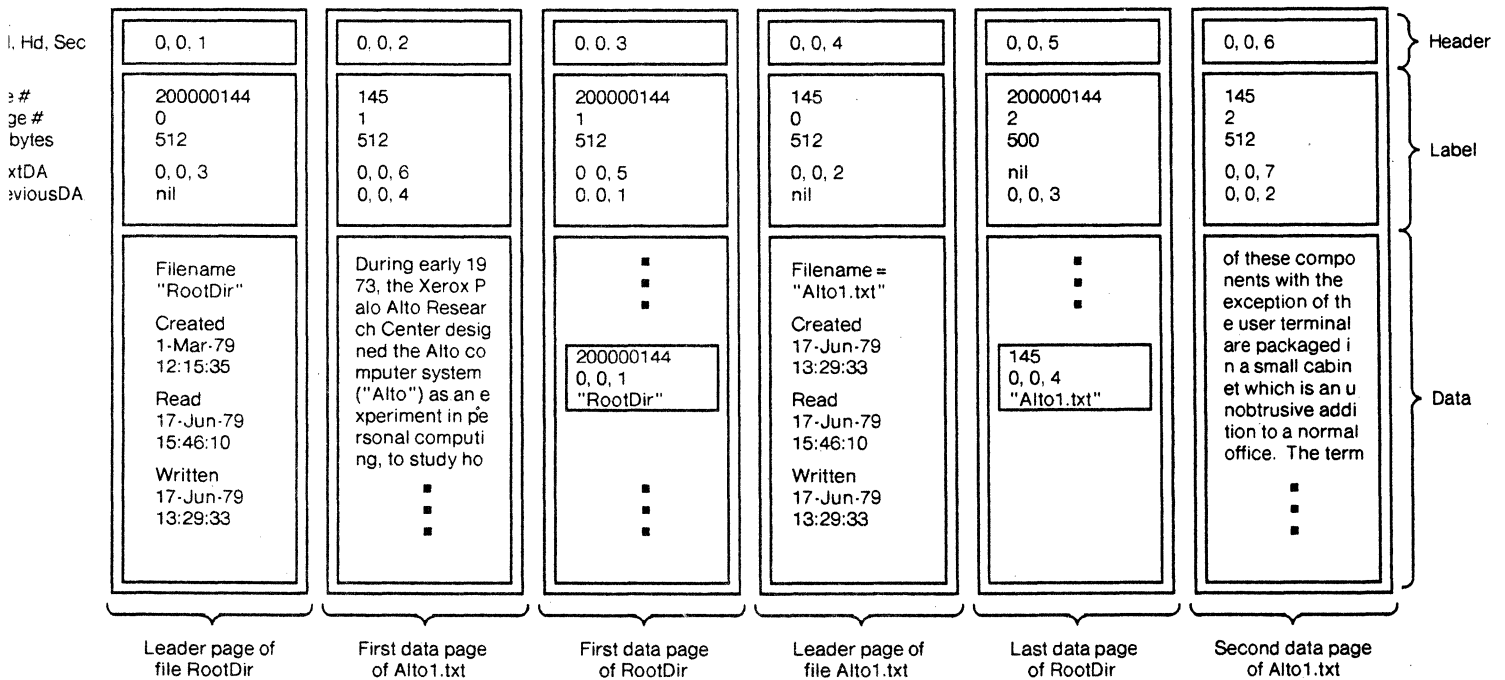
Figure 10. The Alto file system structure.
